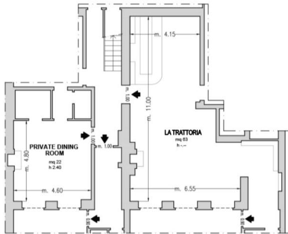
Piano -1 / Basement
